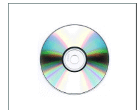
Software
